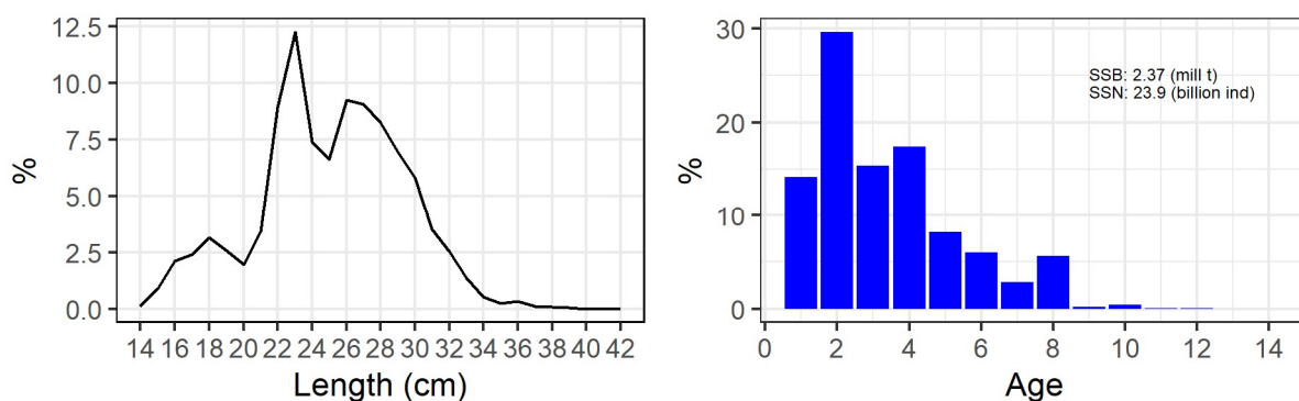
Figure 12. Length and age distribution (numbers) of total stock of blue whiting. March-April 2022.
