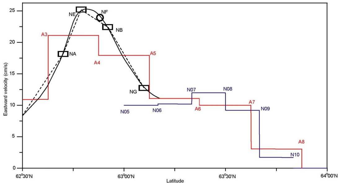
Figure 2.4.4 Values for the altimetry offset U_k^0 (red line) plotted together with altimetry-corrected (Table 2.4.1) average values for surface velocity from the four long-term ADCP sites (rectangles) and surface velocity from average geostrophy (Table 2.4.3) (blue line). Dashed and full black lines show two different ways to interpolate between ADCP sites.
