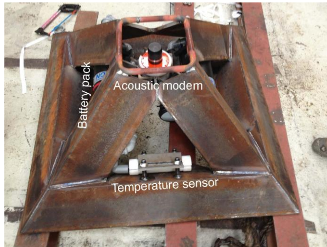
Figure 9.2.1 A trawl-proof unit for measuring bottom temperature. The unit has a SeaBird SBE39 temperature sensor that measures and stores temperature every hour connected to a LinkQuest acoustic modem UWM2000, both of which are powered by two battery packs designed to power the unit > 5 years.
