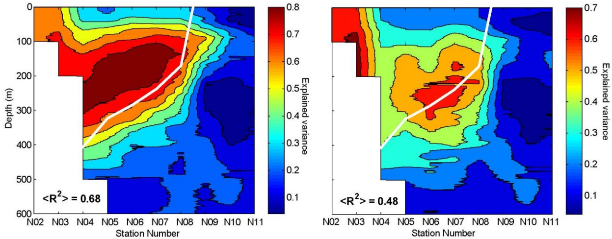
Figure 4.8.2 Explained variance ( R^2 ) of the salinity field. Left: Explained variance of the observed salinity field by Eqs. (4.8.1) and (4.8.2) with observed d_d(k, t_m) and S_{Atl}(t) . Right: Explained variance of the observed salinity field by Eqs. (4.8.1) and (4.8.2) with S_{Atl}(t) and simulated d_d(k, t_m) . The value given for \langle R^2 \rangle on each panel is the average over the average Atlantic water extent, which is bounded by the thick white line on each panel.
