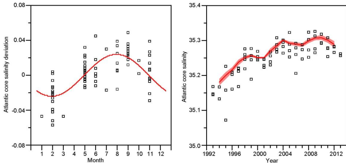
Figure 4.7.1 Salinity variations of the Atlantic core. Left panel: Seasonal variation of the deviation from the 3-year running mean of the Atlantic core salinity. Each square represents one cruise. The red curve is the fitted sinusoidal seasonal variation. Right panel: Each square represents the observed Atlantic core salinity from one cruise. The red curve is the 3-year running mean deseasoned salinity with the red background colour representing \pm one standard error.
