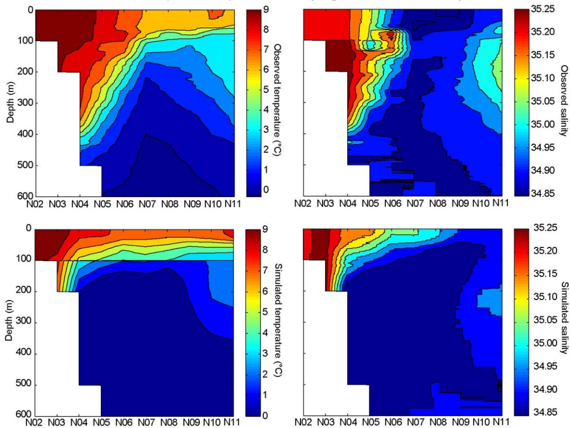
Figure 4.8.3 Temperature (left panels) and salinity (right panels) on cruise 1236, 7 October 2012, as observed (top panels) and as simulated (bottom panels). Unrealistically low temperatures and salinities in the simulated fields have been adjusted to minimum values.
