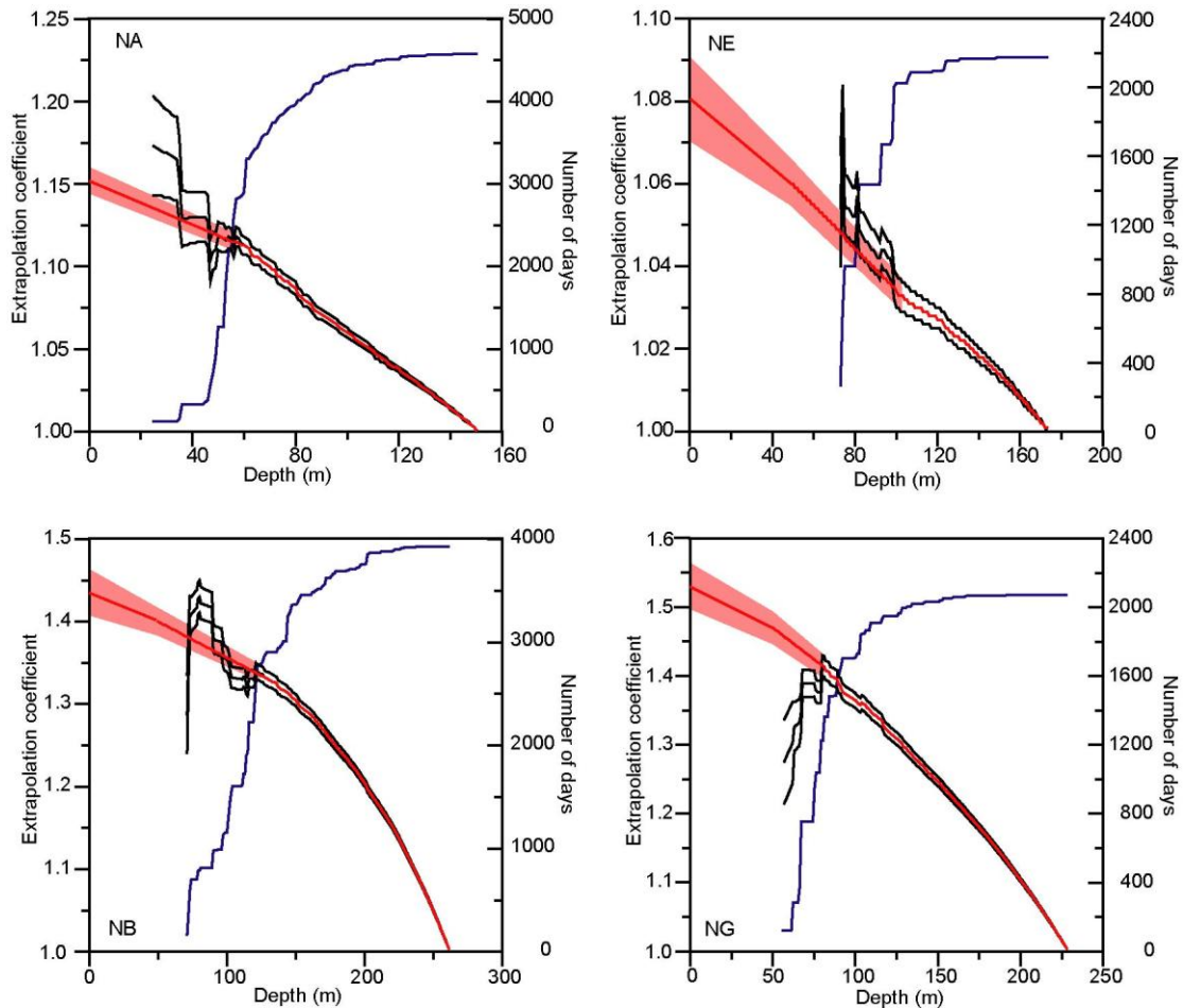
Figure 2.2.2 Vertical extrapolation factors for the long-term ADCP velocities. Each panel shows for one of the long-term ADCP sites, the number of days with data at each depth (blue curve, right scale) and the extrapolation factor \alpha(z) as observed (black lines \pm standard error) and extended (red curve, left scale). The extension up to the surface was based on average geostrophic profiles and extrapolation by eye. The semitransparent red area indicates an uncertainty range extended by eye up to the surface.
