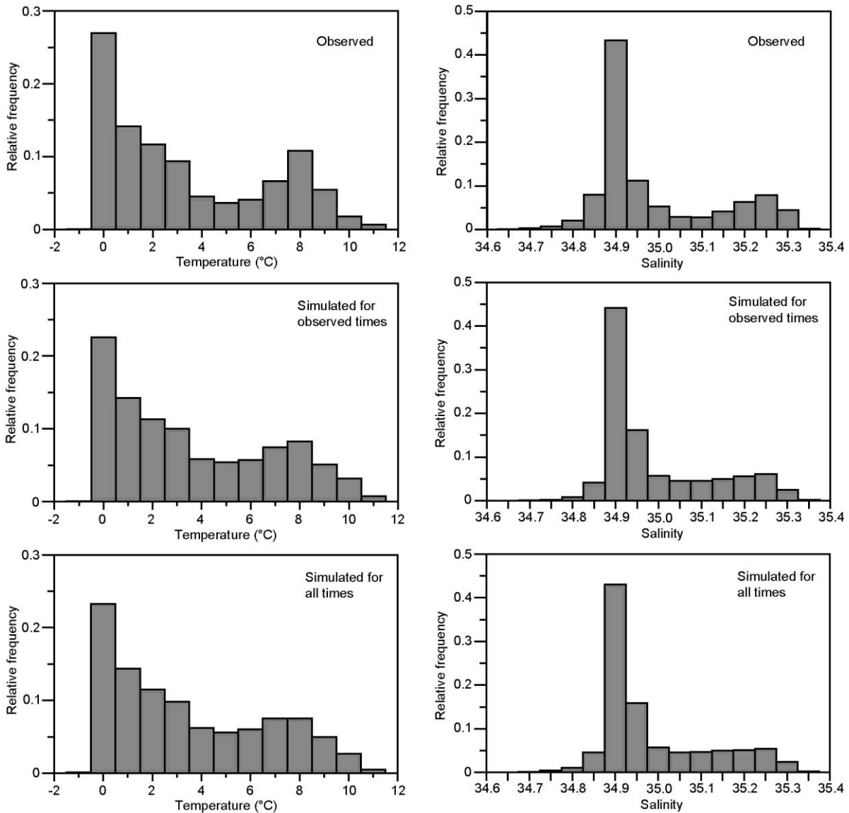
Figure 4.8.4 Histograms of temperature (left) and salinity (right). For every standard station N02 to N11 and for every meter down to bottom or 600m, the relative occurrence of temperatures and salinities are shown as observed on the 78 CTD cruises (top panels), as simulated for the days of the cruises (middle panels), and as simulated for each day in the altimetry period (bottom panels).
