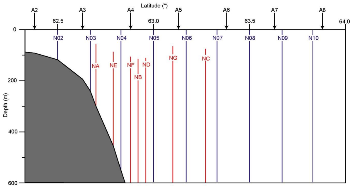
Figure 2.1 The observational section along 6.083^{\circ}\text{W} . CTD standard stations N02 to N10 are marked by blue lines. ADCP profiles are marked by red lines that extend up to the depth, at which 50% of the daily averaged profiles are valid. Altimetry points A_2 to A_8 along 6.125^{\circ}\text{W} are marked by black arrows. See Appendix A for details.
