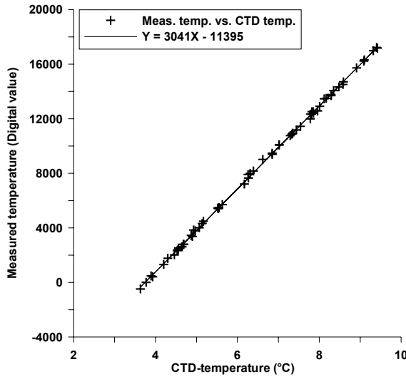
Figure 4.2. Calibration of measured SST (from approx. 3 m depth) vs. CTD surface temperature (from 3-5 m depth) on cruise 9932.
