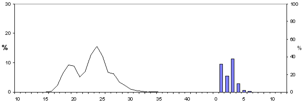
Figure 3.5.6 Length (cm) and age (years) distribution of blue whiting in the Faroese EEZ and Norwegian Sea in May 2003. Based in the acoustic results from R/V “Magnus Heinason”, R/V “Arni Fridriksson”, and R/V “G.O. Sars”, and biological data from R/V “Magnus Heinason” and R/V “G.O. Sars”.
