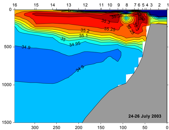
Figure 3.1.13 Salinity in the Svinøy section, 24-26 July.
