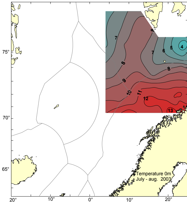
Figure 3.1.15 Surface temperature in July/August 2003.
