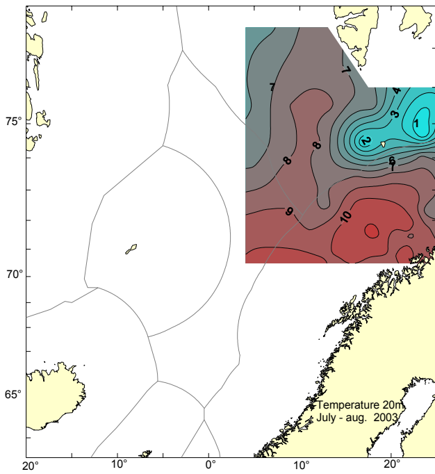
Figure 3.1.16 Temperature at 20 m depth in July/August 2003.
