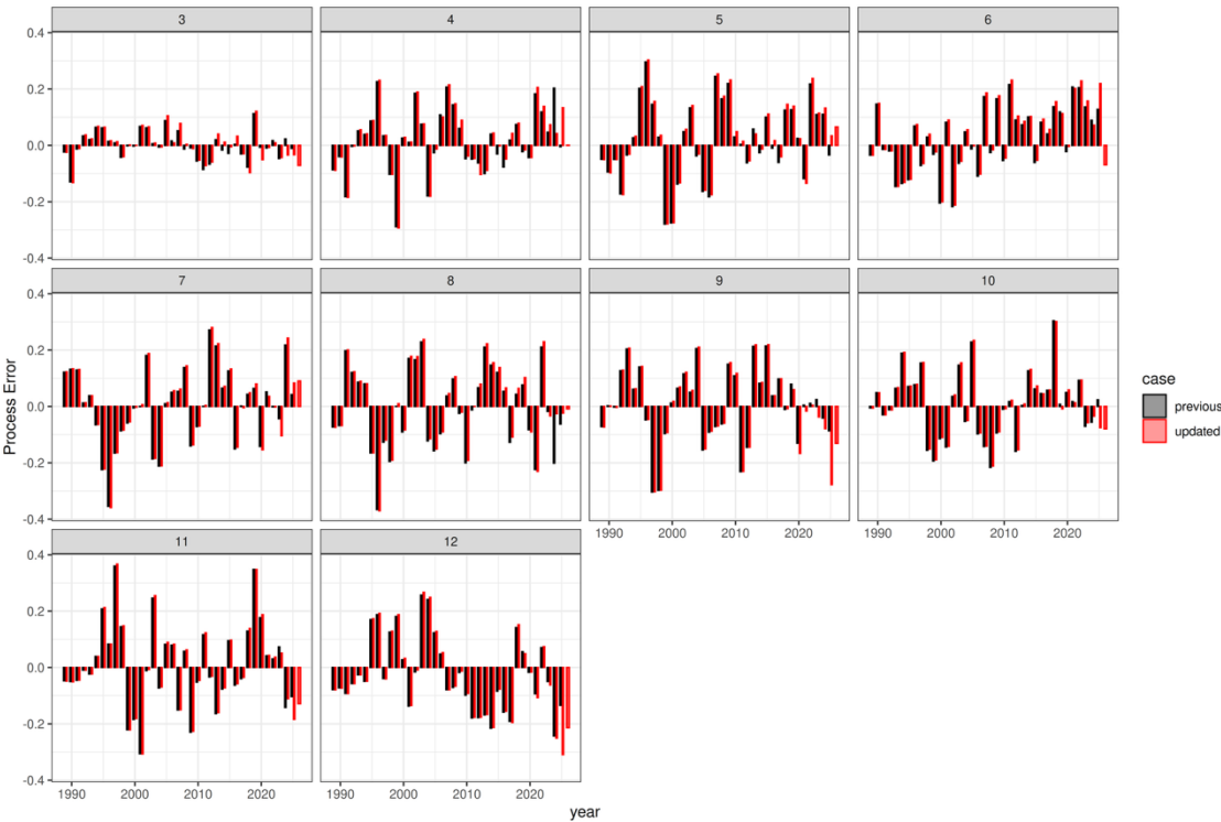
Figure 4.5.1.8. Norwegian spring spawning herring. Comparison between the process error from the 2026 assessment and the 2025 assessment.
