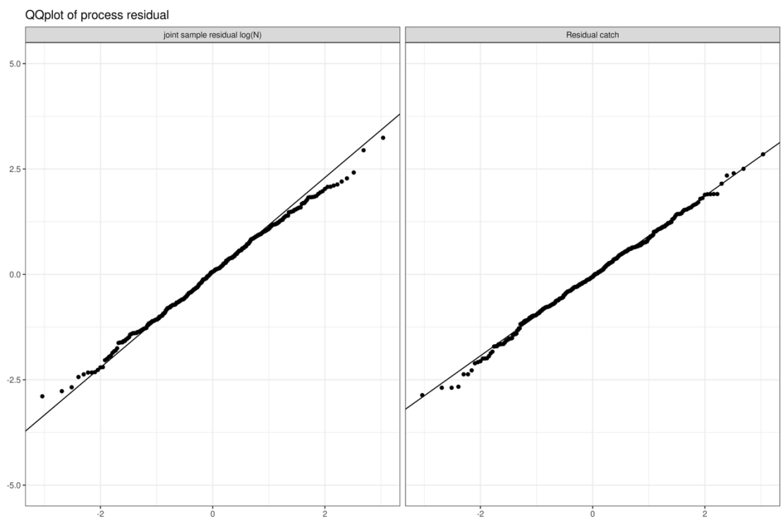
Figure 4.5.1.7. Norwegian spring spawning herring. The corresponding QQ-plot for the process residual in figure 4.5.1.6.
