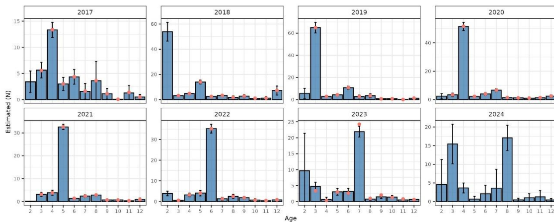
Figure 4.4.7.8. Yearly tag-based abundance estimates at age for NSSH based on the Lincoln Petersen model ( N = R * N_{scan} / r ). Estimates are means with 95 % CIs from bootstraps with 1000 iterations based on R of an age in a release year, and N_{scan} and r of the same year class in YearsOut = 1-2 after release. Age 12 is plus group. Note that red dots represent last year's official input (WGIDE 2025) data for comparison. Small adjustments of 2023 estimates are linked to the addition of one more year with N_{scan} and r . Estimates are only based on N_{scan} and r from factories and periods with accepted efficiencies.
