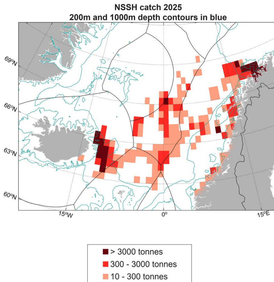
Figure 4.2.1.1. Total reported landings (ICES estimates) of Norwegian spring-spawning herring in 2025 by ICES rectangle. Landings below 10 tonnes per statistical rectangle are not included.
