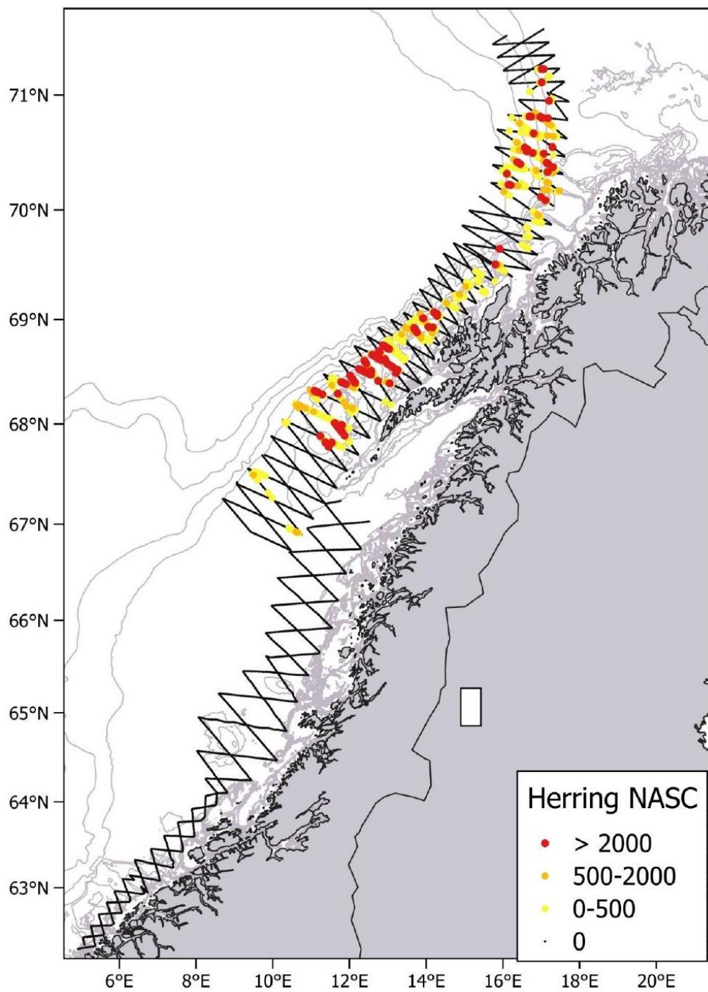
Figure 4.4.7.2. Norwegian acoustic survey on the NSSH spawning grounds. Distribution and acoustic density of herring recorded in 2026.
