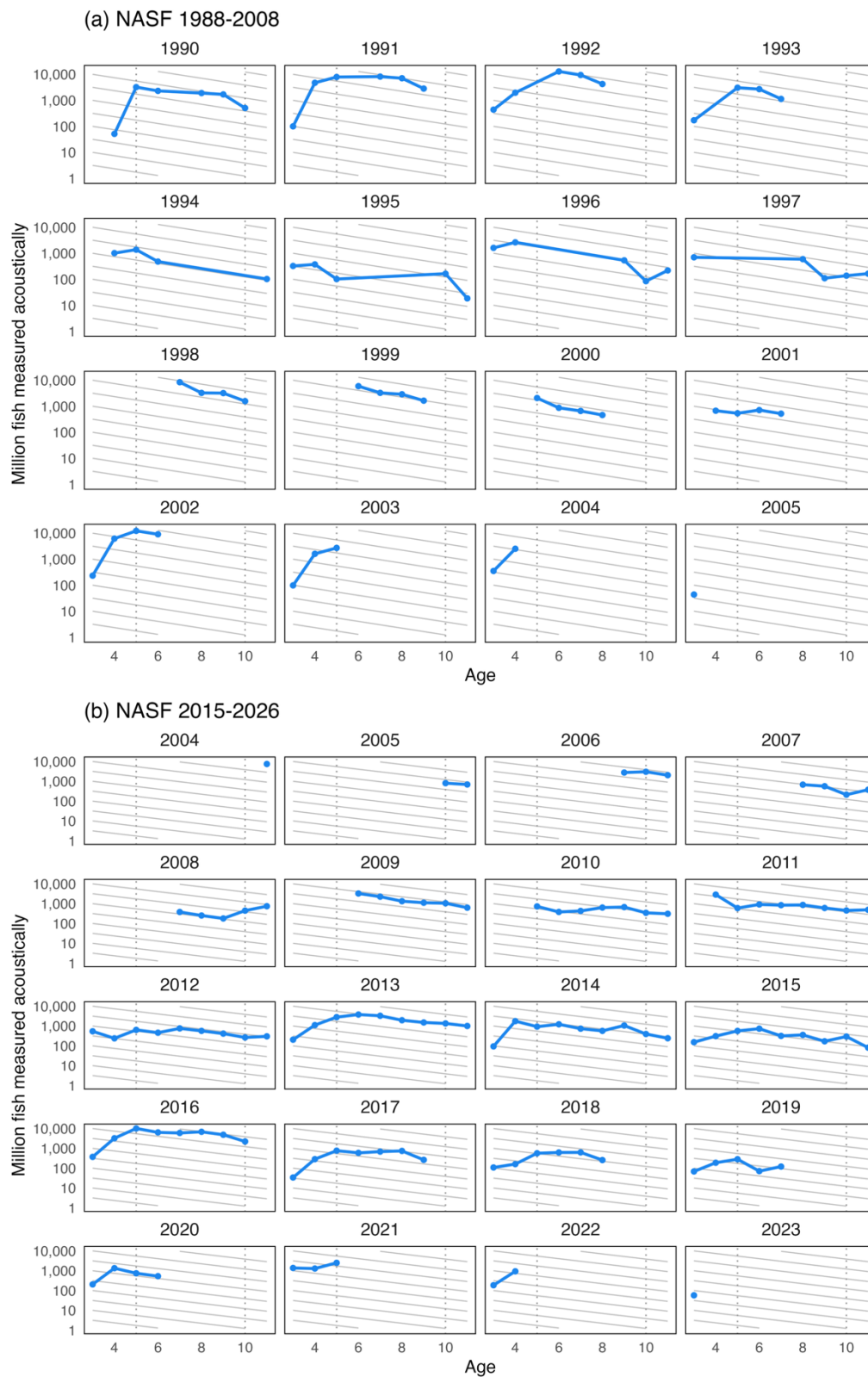
Figure 4.4.7.3. Norwegian spring spawning herring. Age disaggregated abundance indices (millions) from the acoustic survey on the spawning area in February-March a) 1988-2008 and b) 2015-2026 plotted on a log scale. The labels indicate year classes and grey lines correspond to Z = 0.3 . Age is on x-axis.
