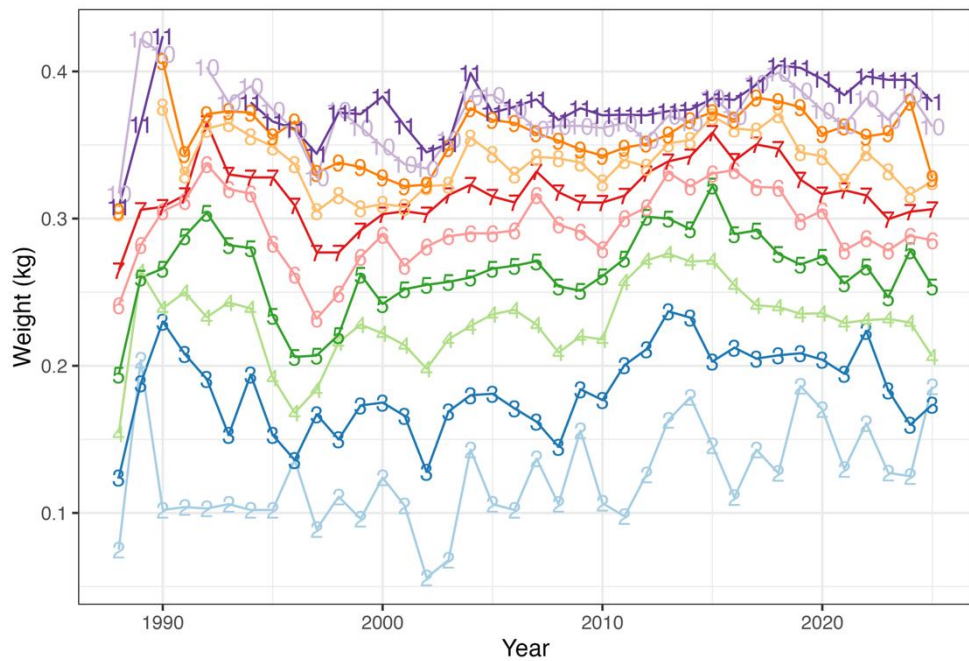
Figure 4.4.4.1. Norwegian spring spawning herring. Mean weight-at-age in catch by age groups 2–11 in the years 1988–2025 in the landings.
