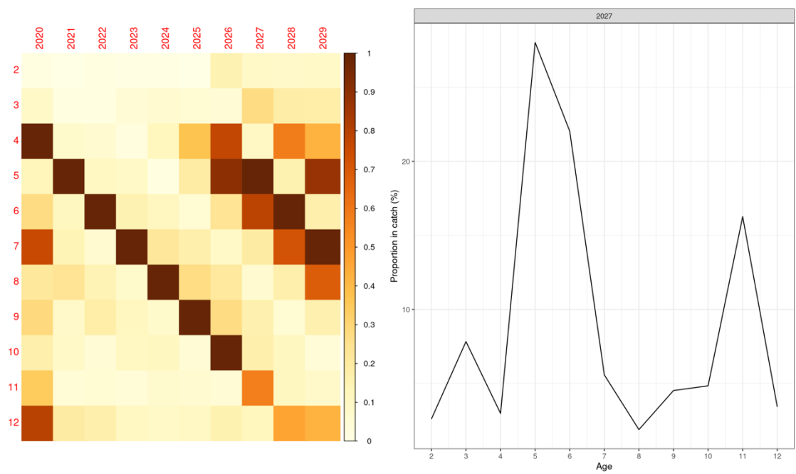
Figure 4.8.1.3 Norwegian spring spawning herring. The observed and predicted catch at age for the year 2020 to 2029 (left). Colours are scaled to the maximum catch withing the year. To the right, the predicted catch at age distribution in 2027.
