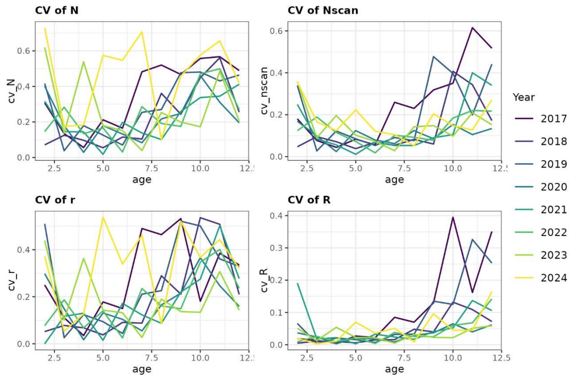
Figure 4.4.7.9. Yearly CVs at age for NSSH for Lincoln Petersen abundance estimates, and for the specific input data to the model ( R , Nscan and r ). CV-estimates are based on bootstraps with 1000 iterations based in YearsOut = 1-2 after release. Age 12 is plus group.
