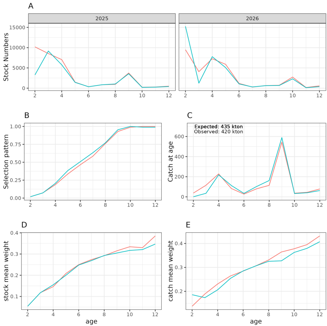
Figure 4.8.3.1. Norwegian spring spawning herring. Comparison between the initial values in the 2025 forecast (red lines) and updated values in the 2026 assessment (blue lines). Panel A show the stock numbers in 2025 and 2026. Panel B show the exploitation pattern, C is the catch-at-age in 2025, D is the stock mean weight, and E is the catch mean weight.
