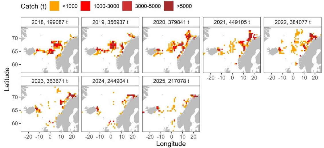
Figure 4.4.7.6. Yearly distributions of catches scanned for tags in NSSH. Note that all catches are included in the maps, also from factories excluded from estimation of the age-based abundance indices due to low efficiency.
