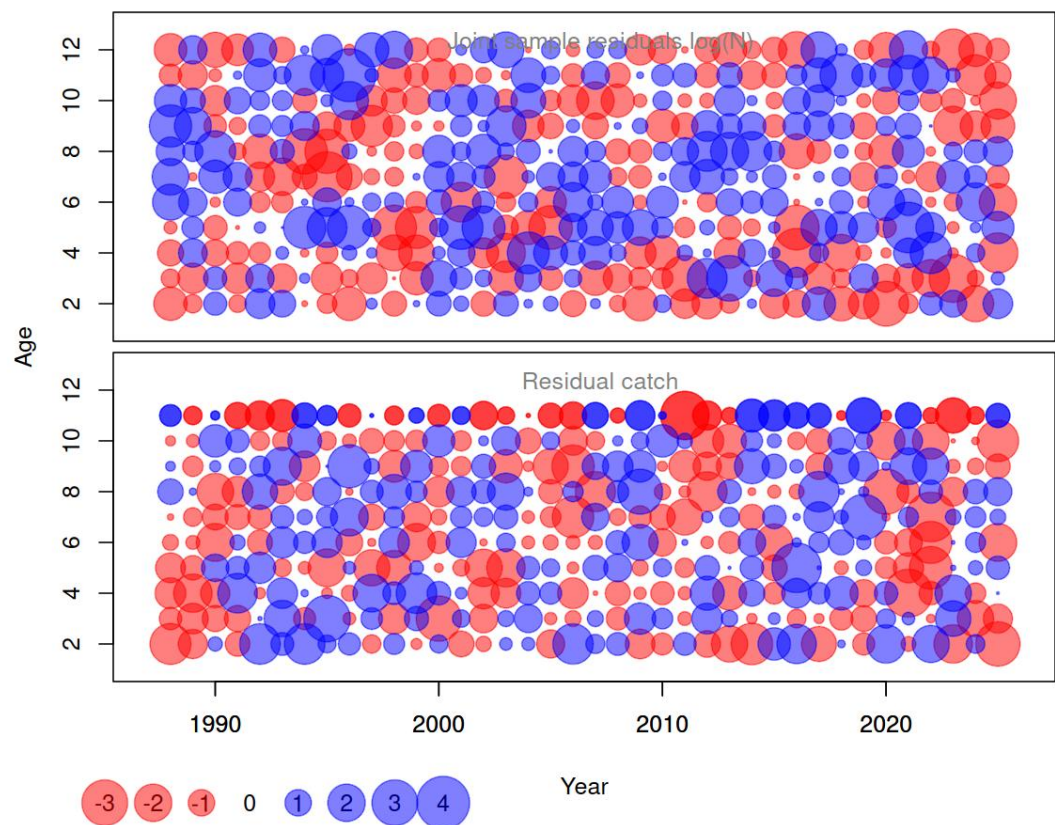
Figure 4.5.1.6. Norwegian spring spawning herring. Process residual for the final model is shown with log(N) in the upper panel and residual catch in the lower panel.
