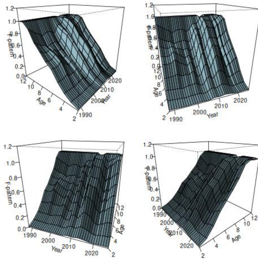
Figure 4.5.1.2. Estimated exploitation pattern for the years 1988–2026 by the SAM model fit. All panels show the same data but are depicted at different angles to improve visibility at various time periods.
