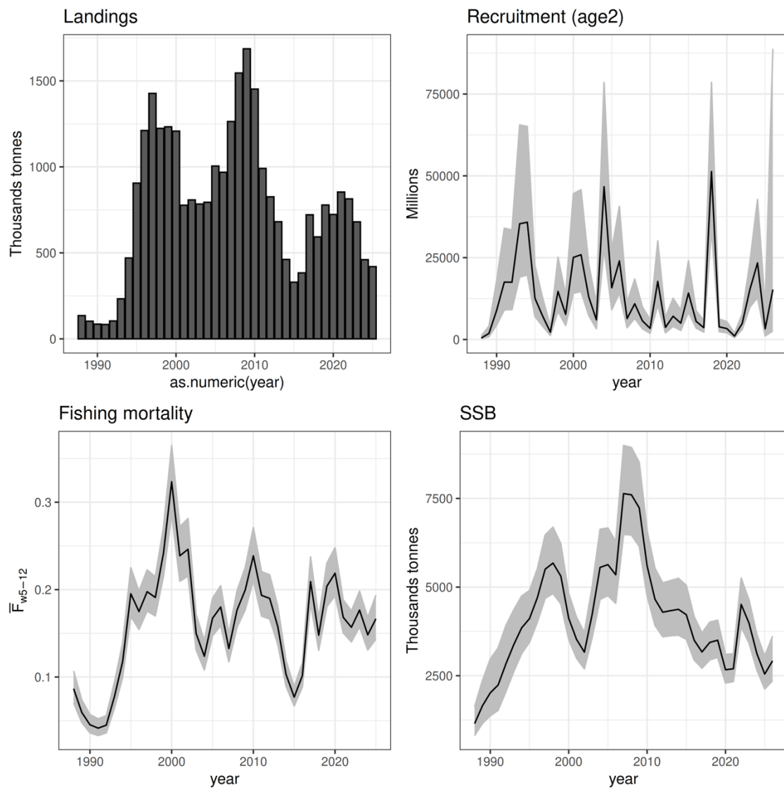
Figure 4.5.1.11. Norwegian spring spawning herring. Total observed landings 1988–2025, estimated recruitment, weighted average of fishing mortality (ages 5–12+) and spawning-stock biomass for the years 1988–2026 based on the final SAM model fit.
