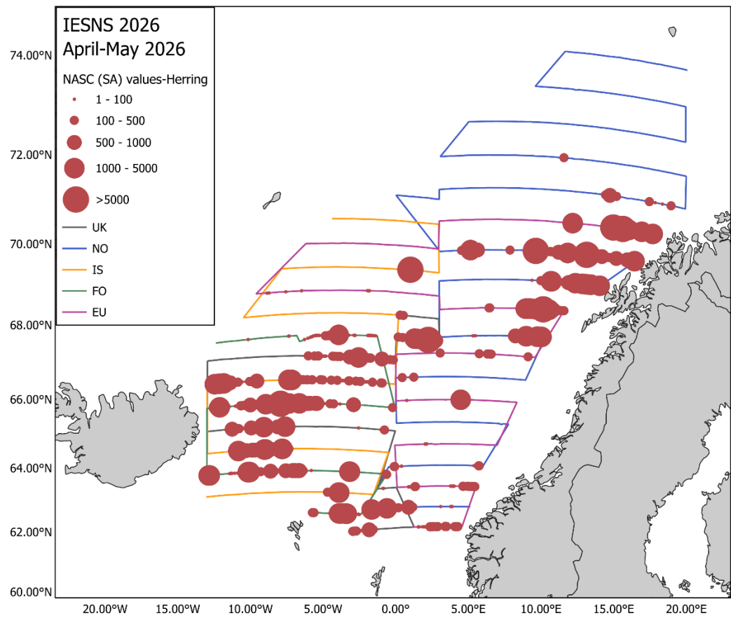
Figure 4.4.7.1. Distribution of Norwegian spring-spawning herring as measured during the IESNS survey in April-May 2026 in terms of NASC values (m²/nm²).
