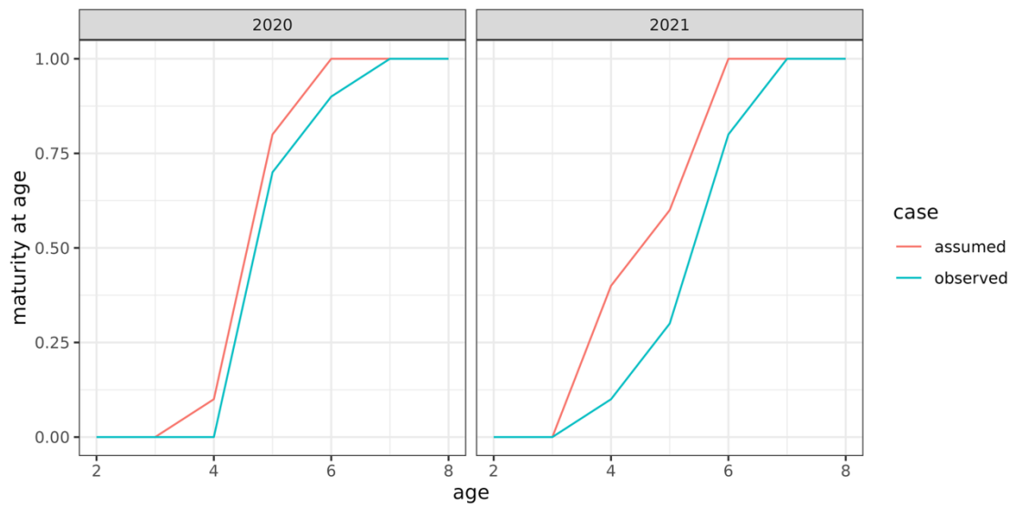
Figure 4.4.5.1. Old assumed (red line) and new back-calculated (blue line) maturity-at-age for the year 2020 and 2021.
