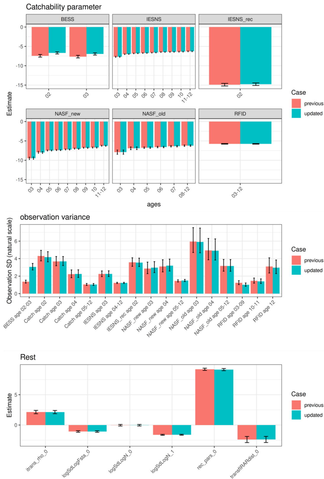
Figure 4.5.1.1. Norwegian spring-spawning herring. A visual representation of parameter estimates of the final SAM model fit. The estimates from the 2025 assessment are also shown (red). Note that in the 2025 assessment external weights was not used for the BESS but included in the 2026 assessment; hence, the observation variance and catchability are different.
