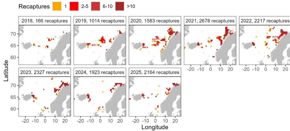
Figure 4.4.7.7. Yearly distributions of recaptured NSSH from releases shown in Fig. 4.4.7.6, and catches shown in Figure 4.4.7.7. All recaptures up to 2025 are included, also recaptures in same year as release (YearsOut = 0 - n) and from factories excluded from estimation of the age-based abundance indices due to low efficiency.
