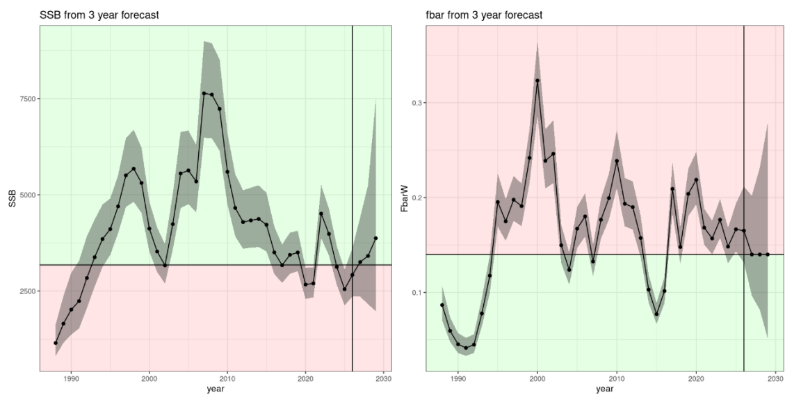
Figure 4.8.1.2 Norwegian spring spawning herring. 3 years predictions on SSB (to the left) and weighted F (to the right), showing the prediction when following the management plan (red field indicates SSB < B_{pa} or F > F_{mgt} ).
