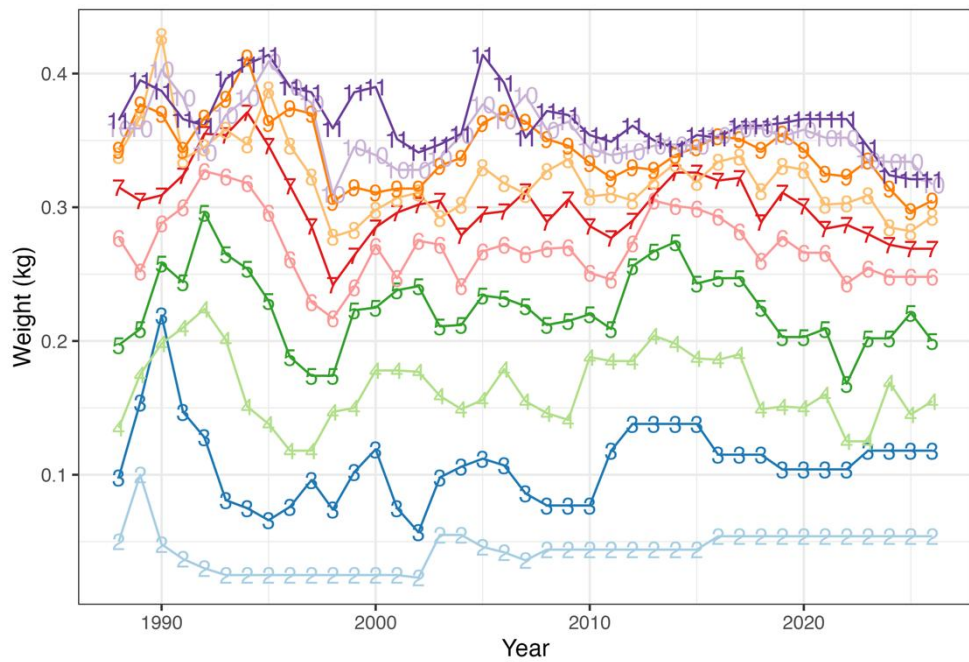
Figure 4.4.4.2. Norwegian spring-spawning herring. Mean weight-at-age in the stock by age groups 2–11 for the years 1988–2026.
