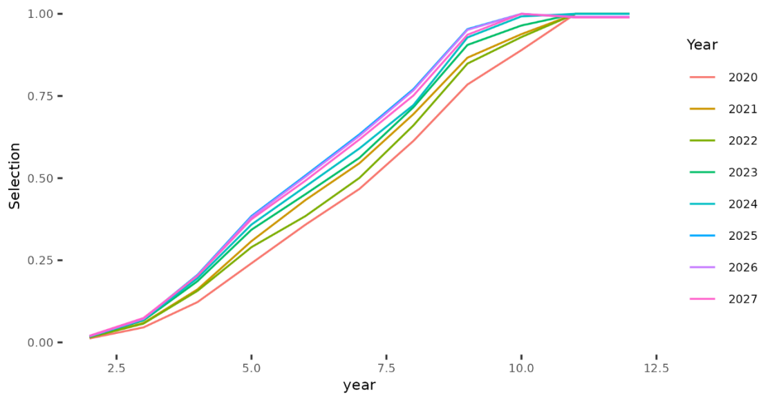
Figure 4.8.1.1. Norwegian spring-spawning herring. SAM estimated selection pattern; selected years (estimates for 2020–2025 and predictions for 2026–2027) are shown in colours as indicated in the legend.
