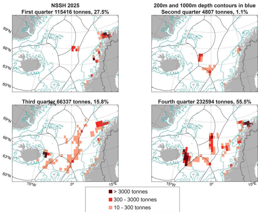
Figure 4.2.1.2. Total reported landings (ICES estimates) of Norwegian spring-spawning herring in 2025 by quarter and ICES rectangle. Landings below 10 tonnes per statistical rectangle are not included.
