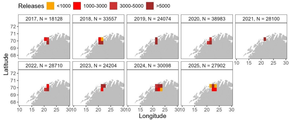
Figure 4.4.7.5. Yearly distributions of tagged NSSH in northern Norwegian fjords. Note that in 2018 the planned November-December survey was postponed to January 2019, but the releases are moved to 2018 both in the map and index.
