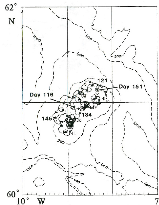
Figure 3. Drogue 3973 during April-May 1987.
